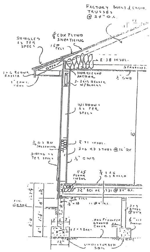
TYPICAL SECTION Figure 1-9
