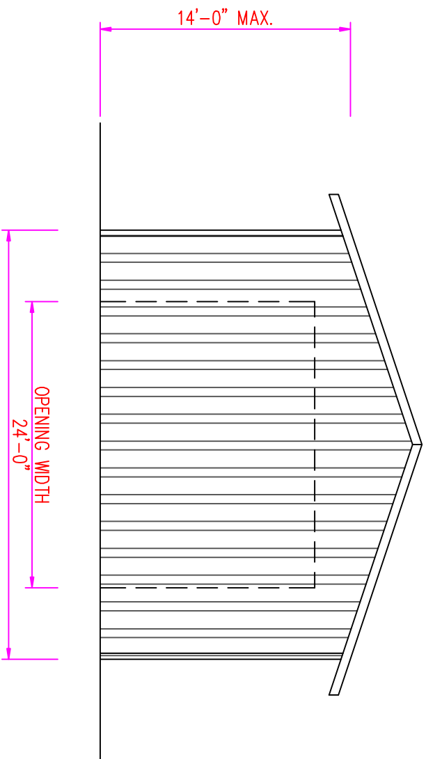
1 S12 GABLE ELEVATION
